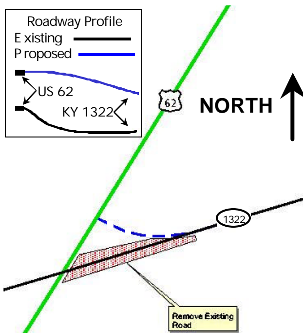
Figure V-12. Recommended Alignment And Profile For KY 1322 at US 62
