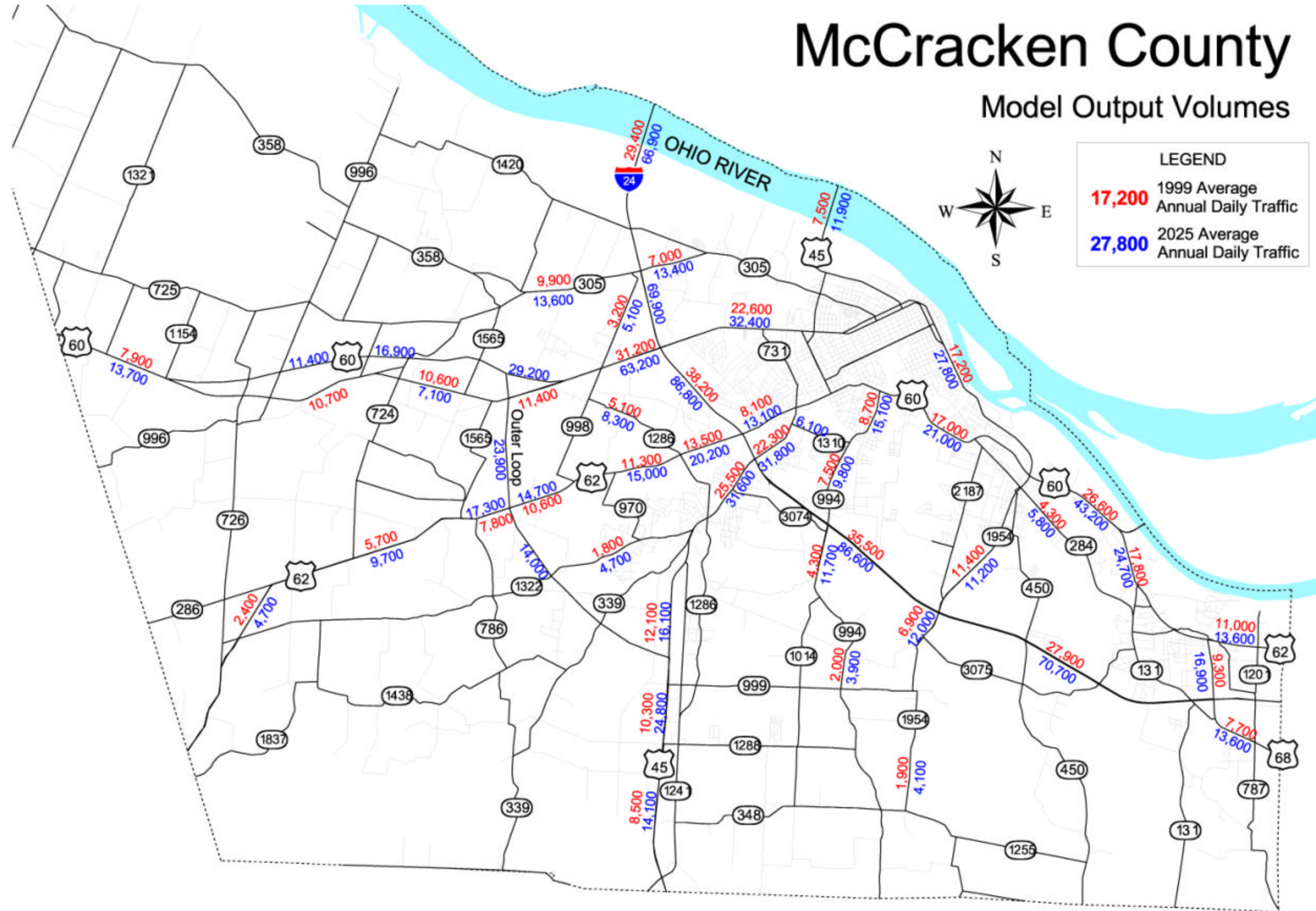
Figure IV- 3. 1999 Existing and 2025 E+C Traffic Volumes
